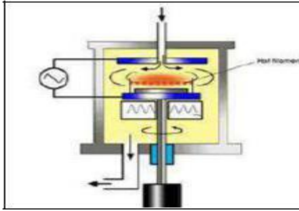
Figure 9 Plasma-enhanced chemical vapor deposition (PECVD) systems
