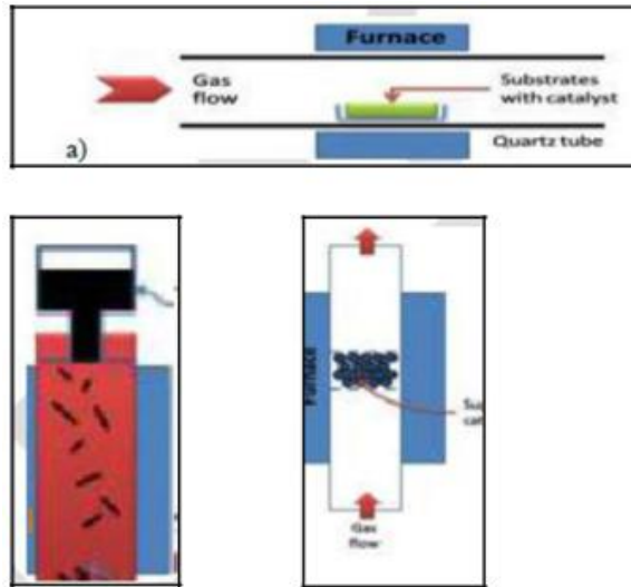
Figure 8: Schematic demonstration of CVD method. (a) Horizontal furnace. (b) Vertical furnace. (c) Fluidized bed reactor.
