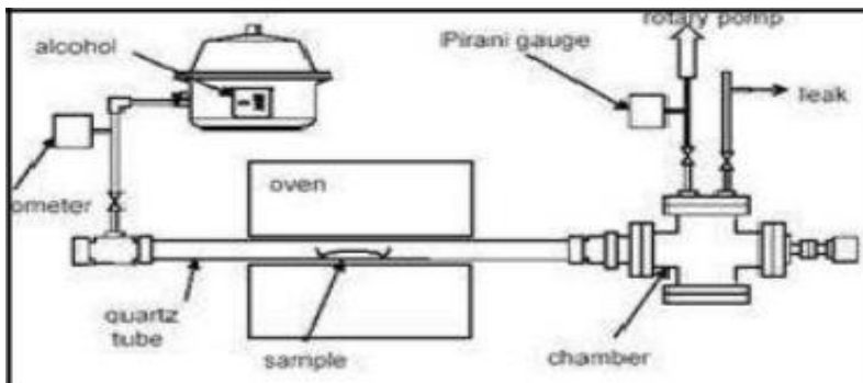
Figure 10: Alcohol catalytic CVD
